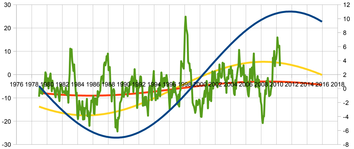
— Sea level — UAH Trop data — Tropical UAH — Solar derived
