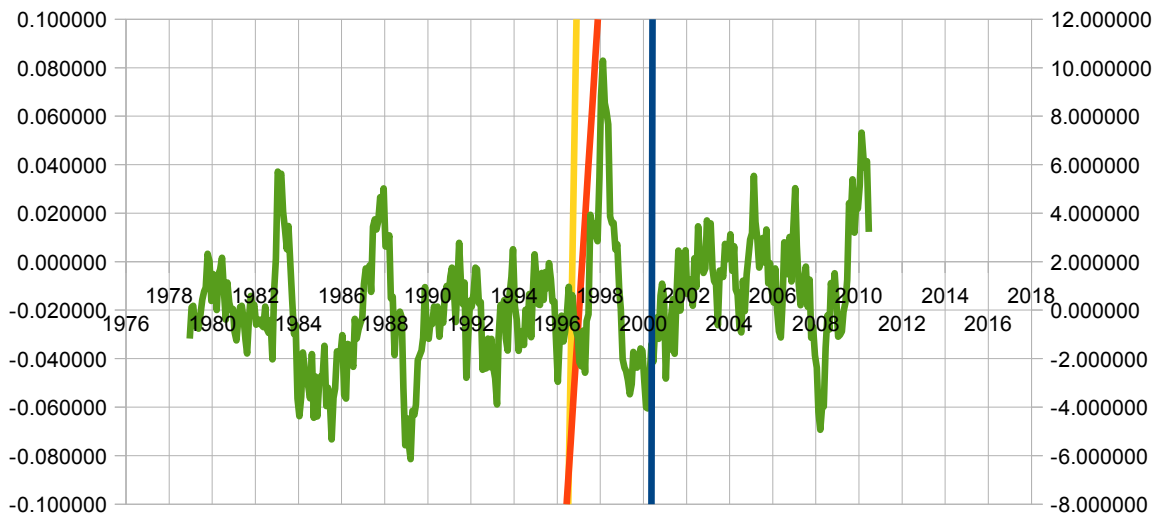
— Sea level — UAH Trop data — Tropical UAH — Solar derived
